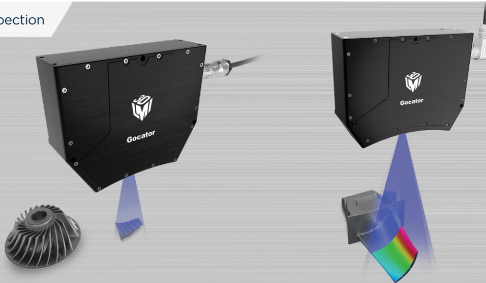
Snapshot sensor capturing surface data of a 3D printed turbine part
